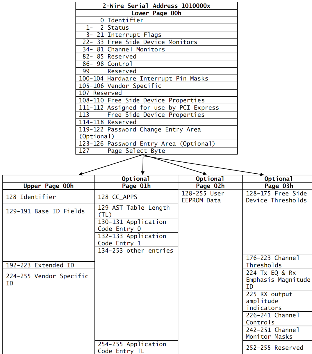
Figure 3, Memory Map
