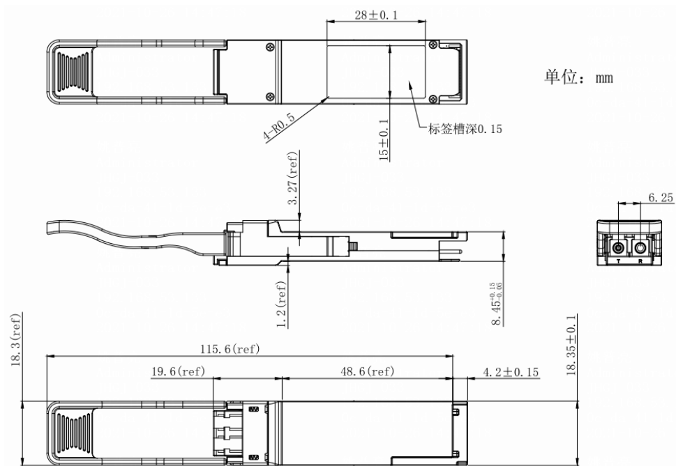
Figure4. Mechanical Outline
