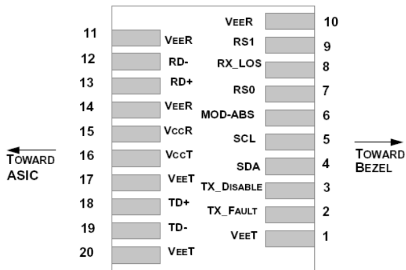
Figure 1, Pin View
