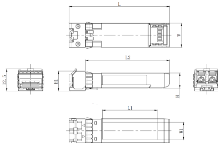
Figure 2, Mechanical Diagram
