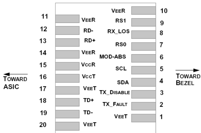
Figure 1, Pin View
